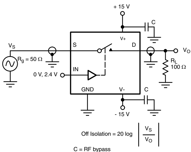
Fig. 5 - Off Isolation
