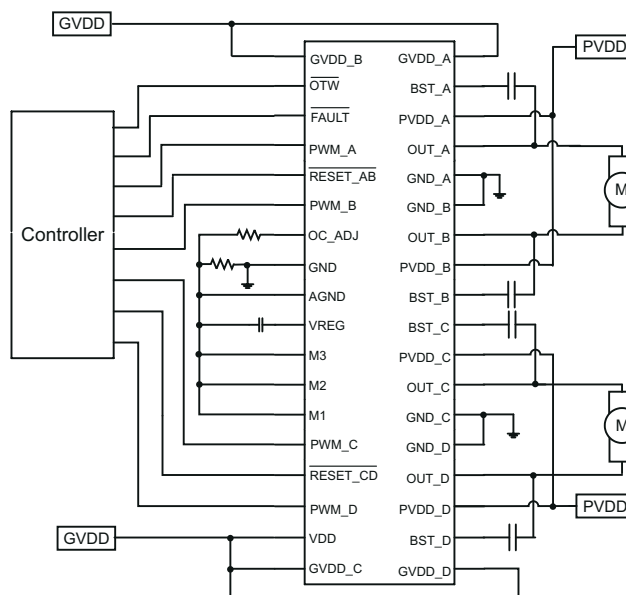
Simplified Application Diagram
