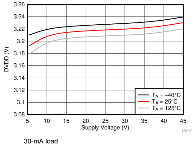
Figure 6-7. DVDD Regulator
