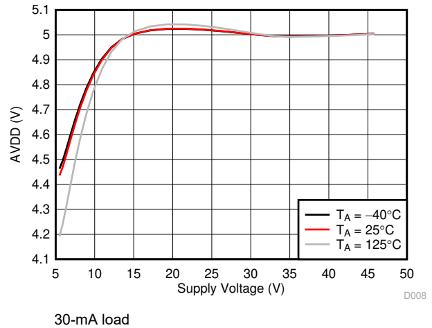
Figure 6-8. AVDD Regulator
