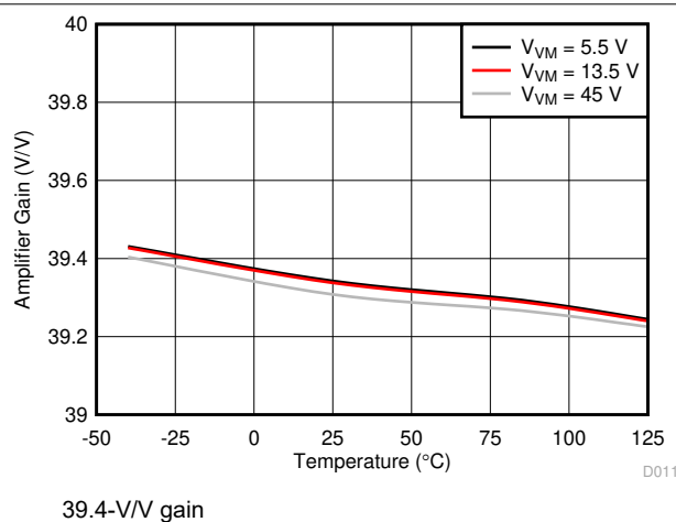
Figure 6-11. Amplifier Gain
