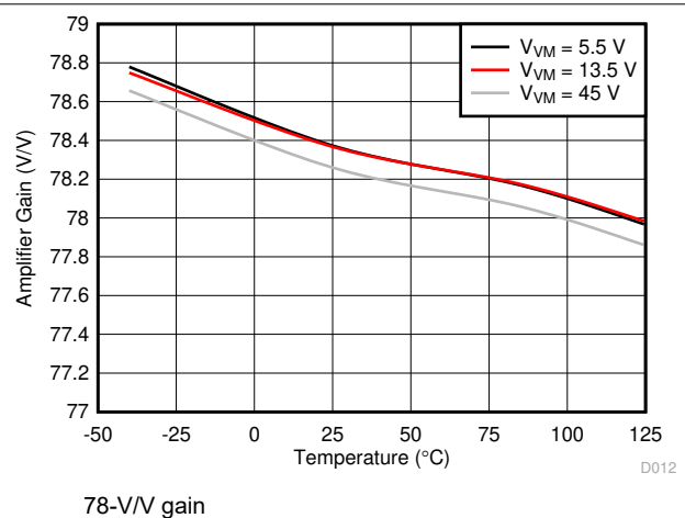
Figure 6-12. Amplifier Gain
