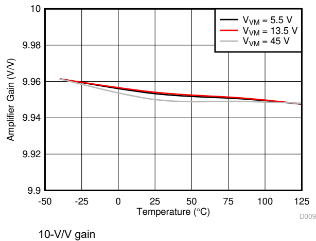
Figure 6-9. Amplifier Gain
