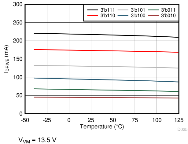
Figure 6-25. Low-Side Source Current
