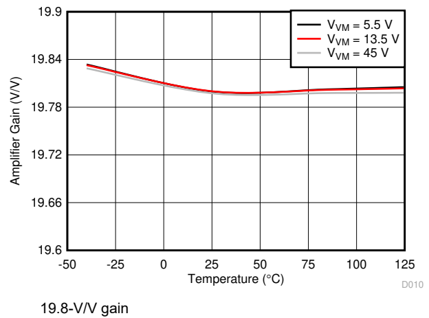
Figure 6-10. Amplifier Gain
