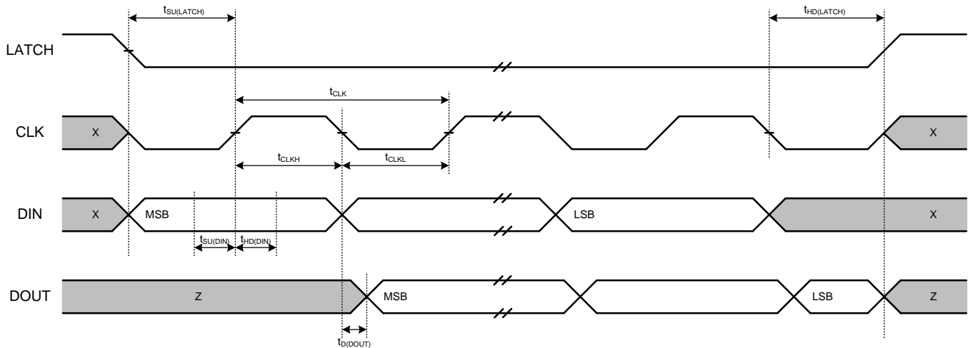
Figure 1. Serial Interface
