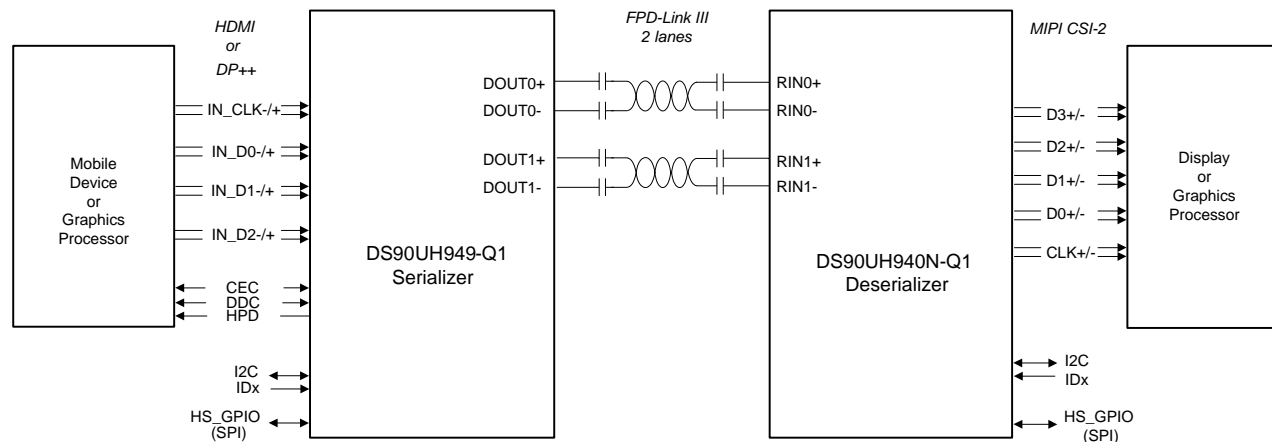
Figure 40. Typical Display System Diagram
