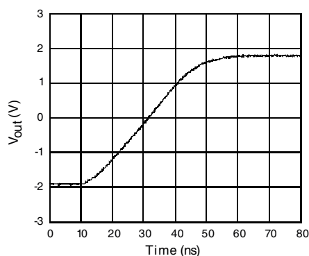
Figure 6. Large signal measurement – positive slew rate ( V_{CC} = \pm 2.5 V) Gain = +2, Z_L = 150\ \Omega // 5.6 pF, V_{in} = 400 mVpk
