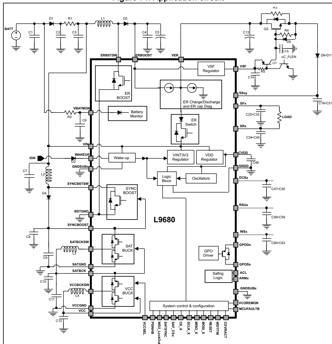
Figure 71. Application circuit
