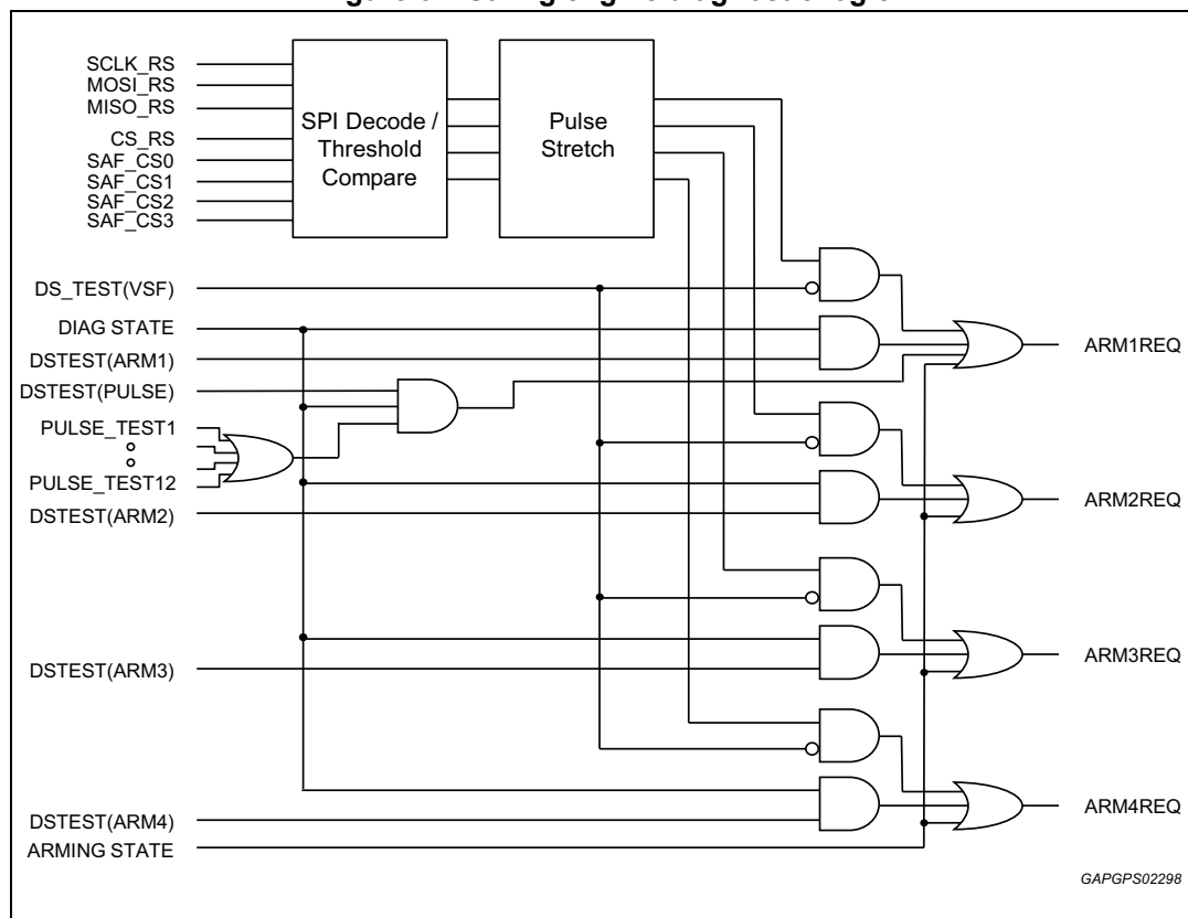
Figure 61. Safing engine diagnostic logic
