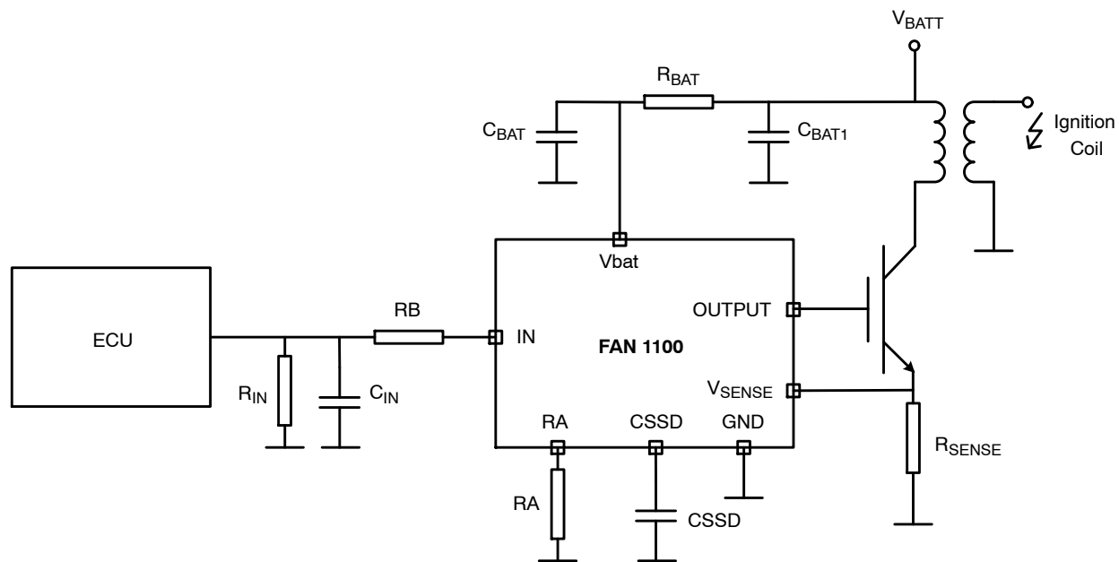
Figure 1. Typical Application
