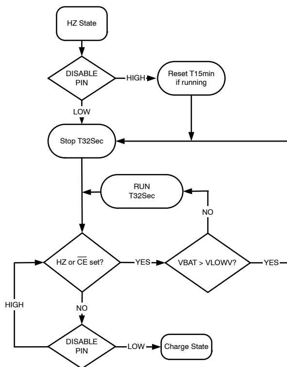
Figure 38. HZ-State
