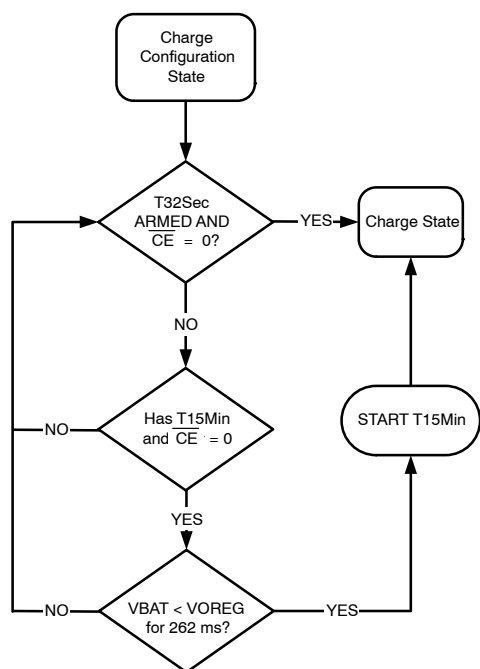
Figure 37. Charge Configuration
