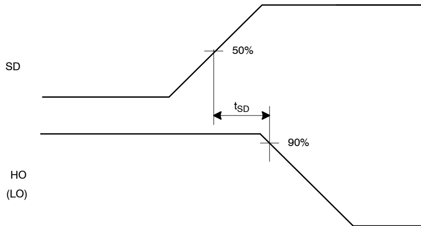
Figure 38. Shutdown Waveform Definition
