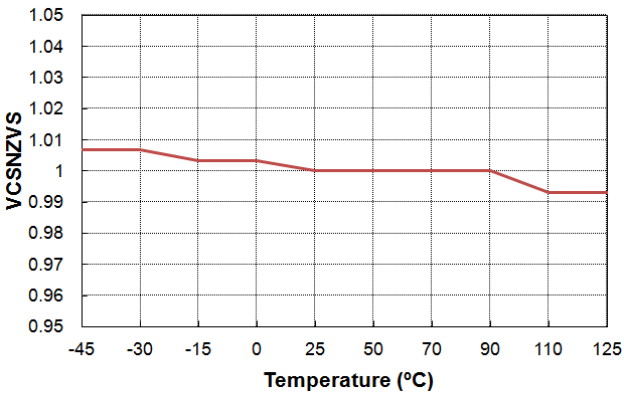
Figure 52. VCSNZVS vs. Temperature
