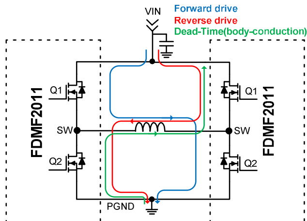
Figure 65. H-bridge Motor Drive
