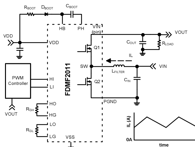
Figure 67. Synchronous Boost Converter Operating in CCM
