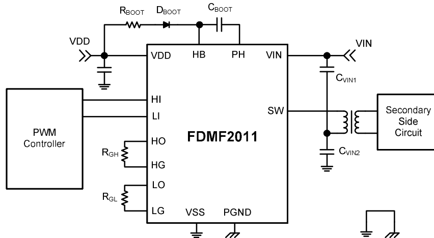
Figure 7. Half-Bridge Converter
