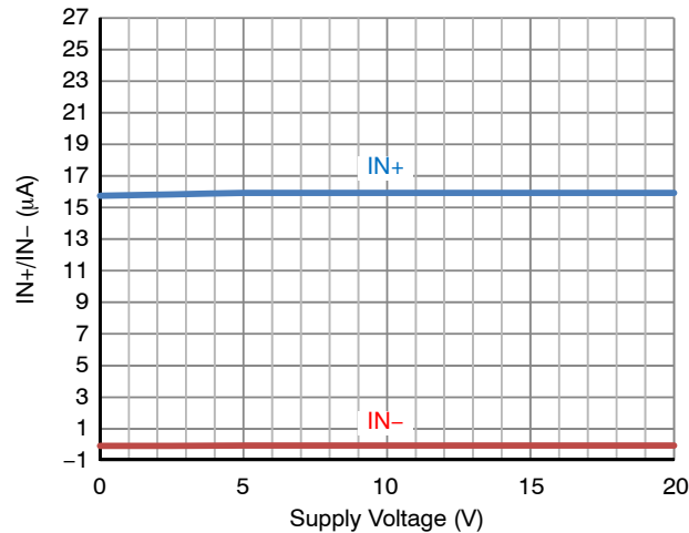
Figure 31. I_{IN+} I_{IN-} vs. Supply Voltage ( V_{DD} )
