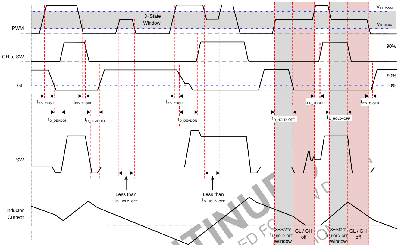
Figure 29. PWM 3-State Timing Diagram (FCCM Held HIGH)
