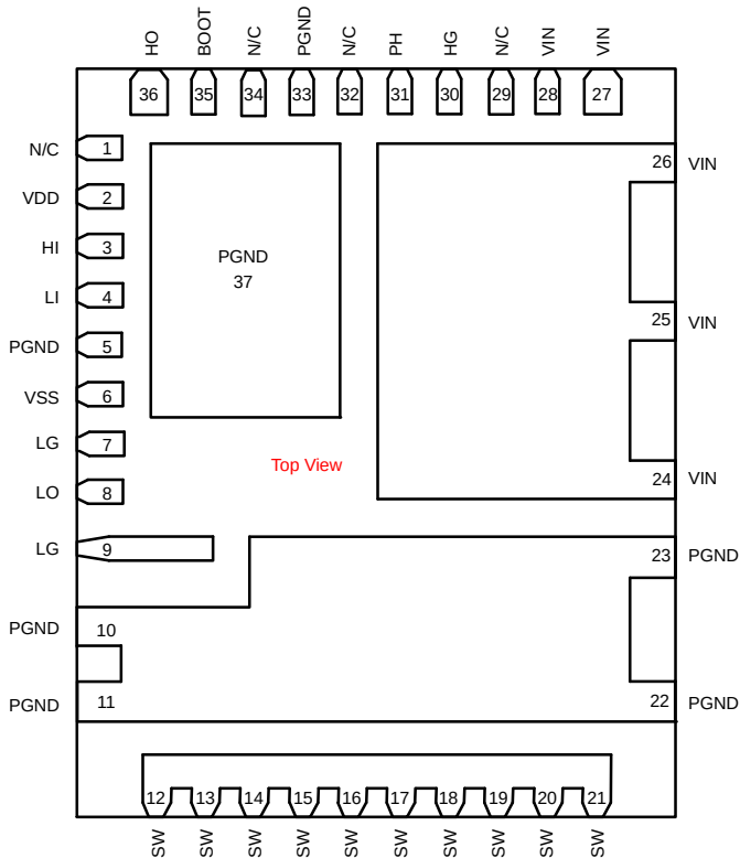
Figure 2. Pin Configuration
