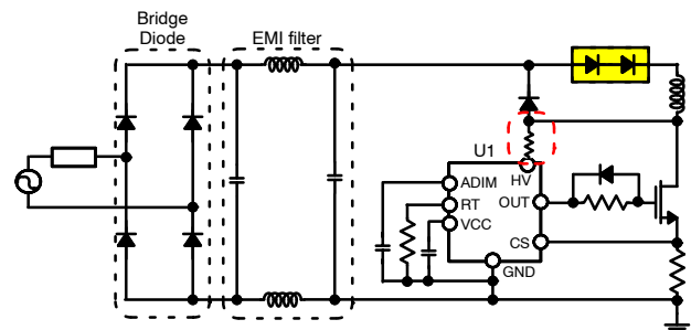
Figure 6. High-Voltage Application
