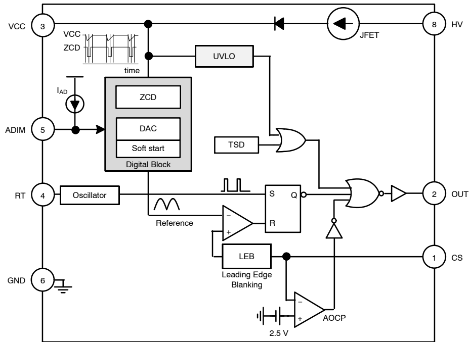
Figure 2. Block Diagram
