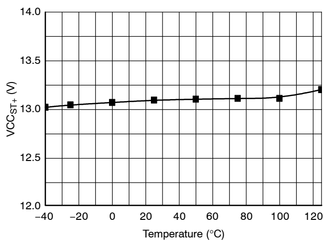
Figure 14. V_{CC_{ST+}} vs. Temperature
