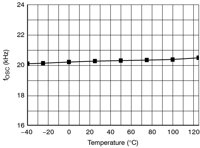
Figure 18. f OSC vs. Temperature (R t = 87 kΩ)
