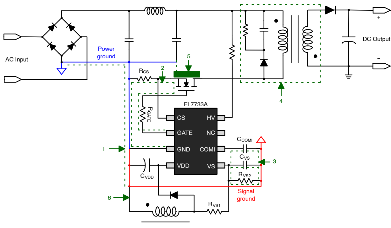
Figure 26. Layout Example
