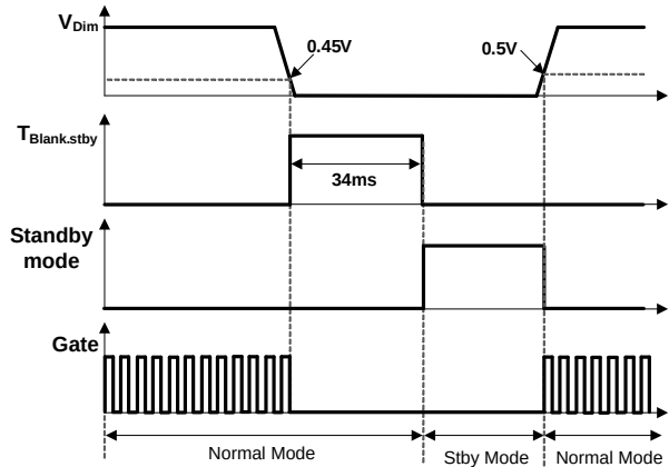
Figure 22. Standby Mode
