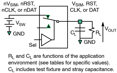
Figure 11. AC Test Circuit Load
