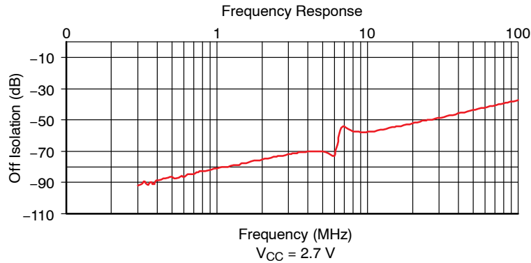
Figure 6. Off Isolation
