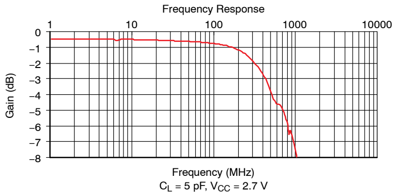
Figure 8. Bandwidth
