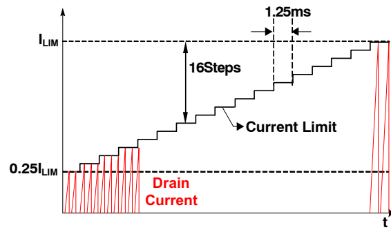
Figure 21. Internal Soft-Start
