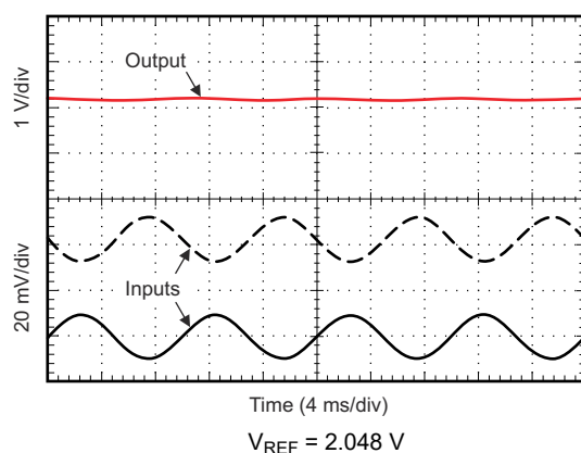
Figure 8-6. Current Differencing Application Output Response (A2 Devices)
