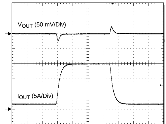
Figure 18. Load Transient Response, 100 \mu\text{s/Div}
