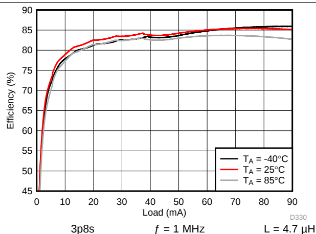
Figure 142. Backlight System Efficiency
