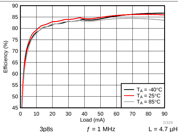
Figure 141. Backlight Boost Efficiency
