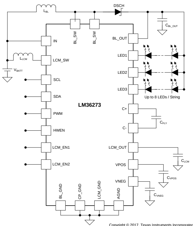
Simplified Schematic
