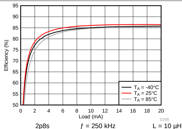
Figure 73. Backlight Boost Efficiency
