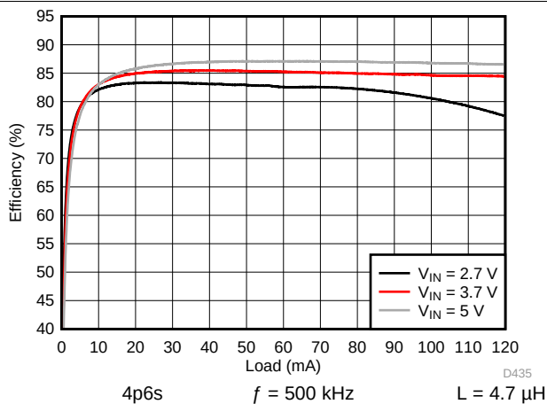
Figure 183. Backlight Boost Efficiency
