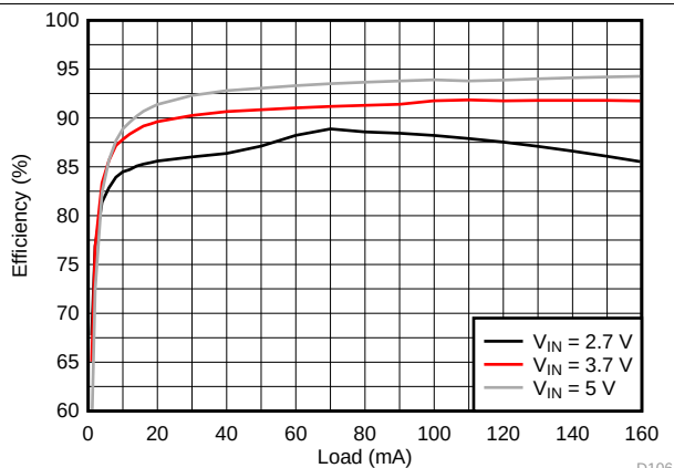
Figure 190. LCM Boost Efficiency
