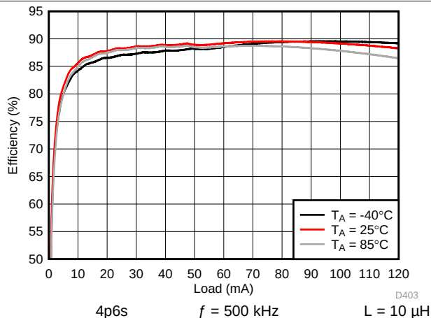
Figure 151. Backlight Boost Efficiency
