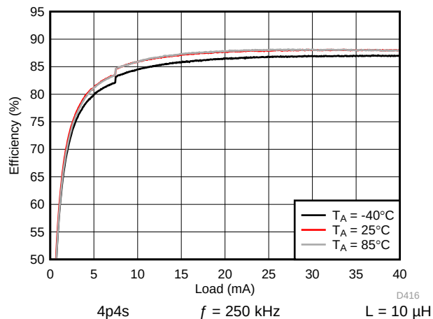
Figure 164. Backlight System Efficiency
