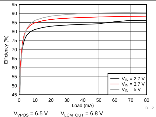
Figure 198. VPOS Efficiency
