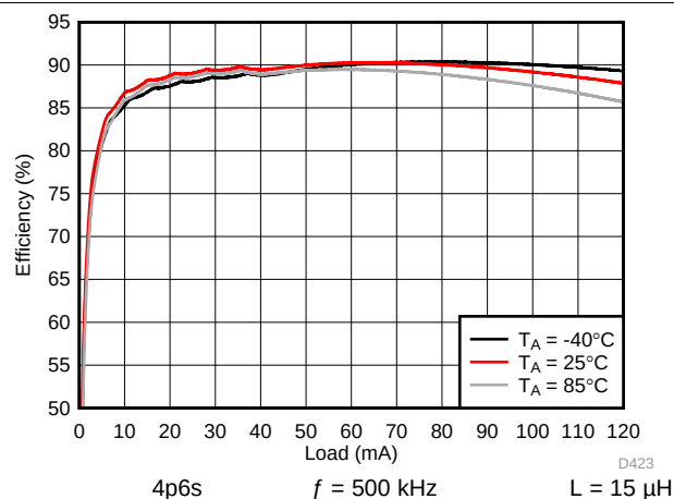
Figure 171. Backlight Boost Efficiency
