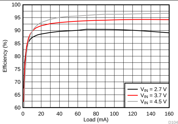
Figure 188. LCM Boost Efficiency
