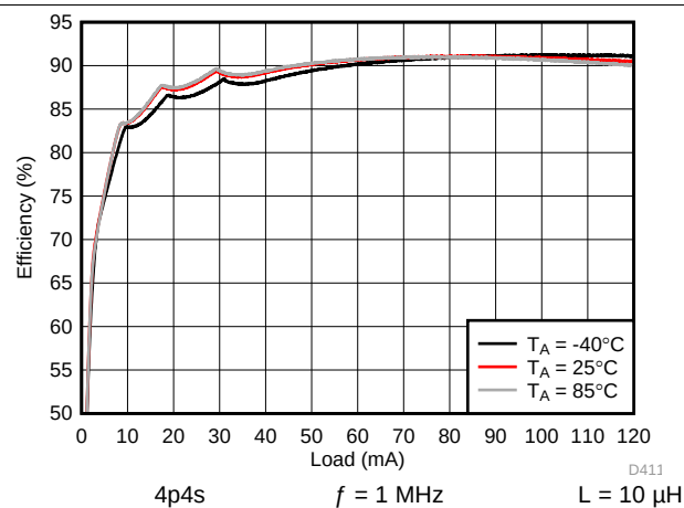
Figure 159. Backlight Boost Efficiency
