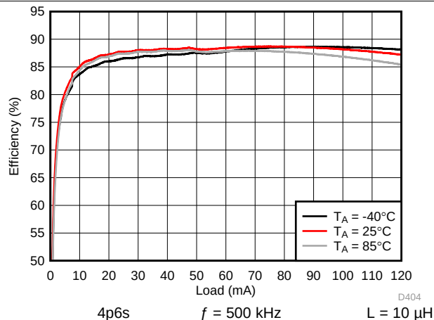
Figure 152. Backlight System Efficiency
