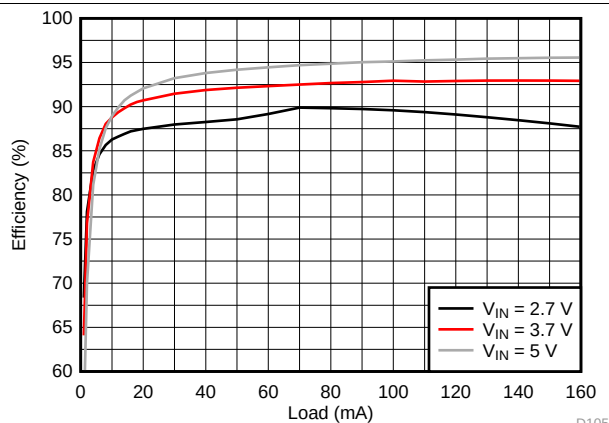
Figure 189. LCM Boost Efficiency
