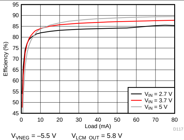
Figure 203. VNEG Efficiency
