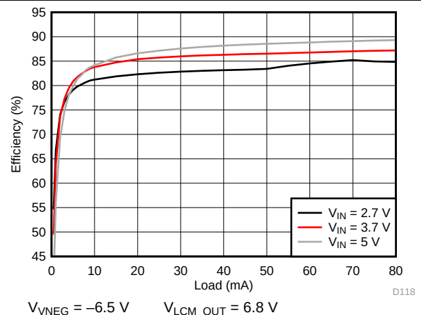
Figure 204. VNEG Efficiency
