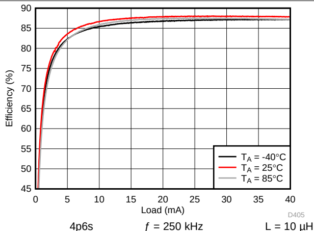
Figure 153. Backlight Boost Efficiency
