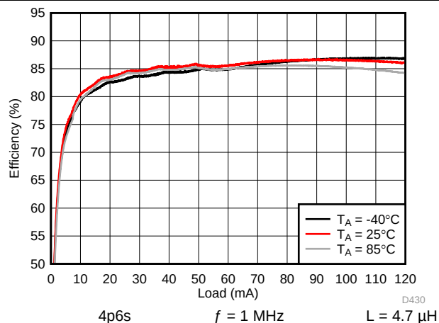
Figure 178. Backlight System Efficiency
