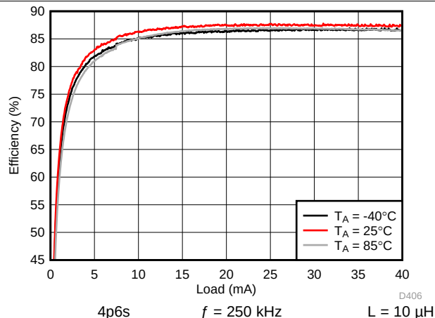
Figure 154. Backlight System Efficiency
