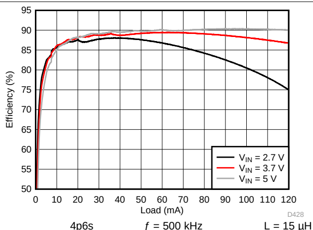
Figure 176. Backlight System Efficiency
