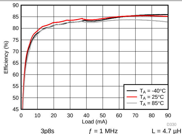
Figure 142. Backlight System Efficiency
