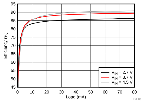
Figure 194. VPOS Efficiency
