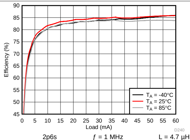
Figure 108. Backlight System Efficiency
