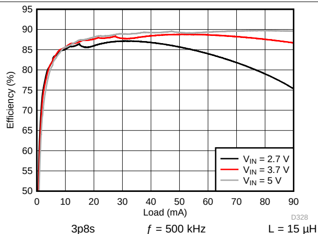
Figure 140. Backlight System Efficiency
