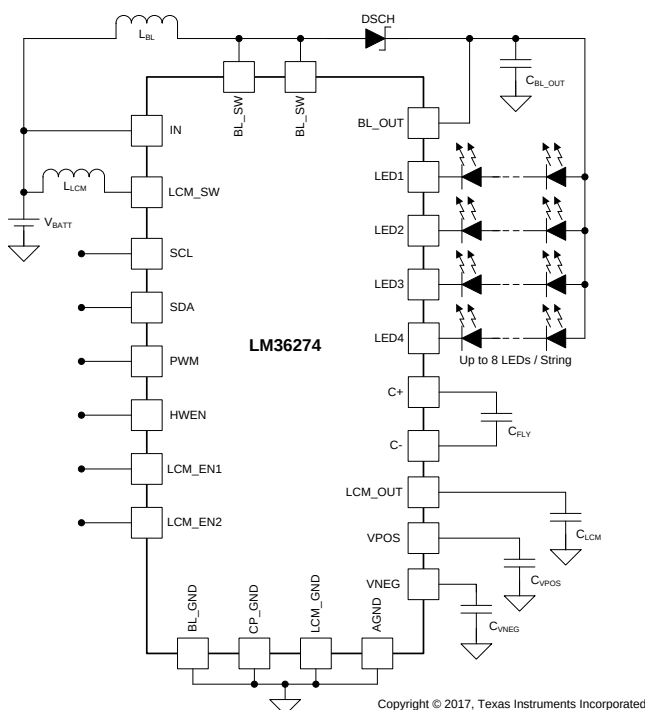
Simplified Schematic
