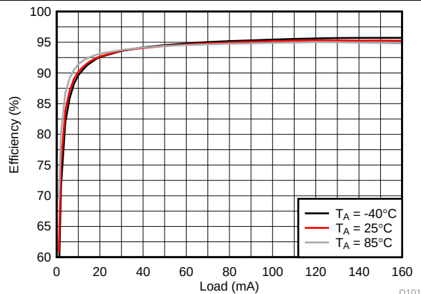
Figure 187. LCM Boost Efficiency
