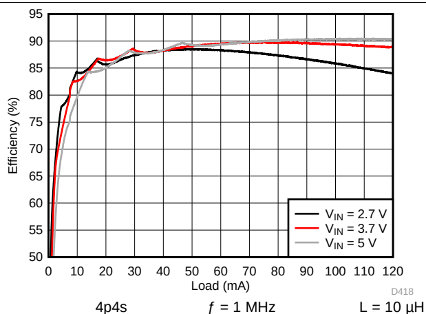
Figure 166. Backlight System Efficiency
