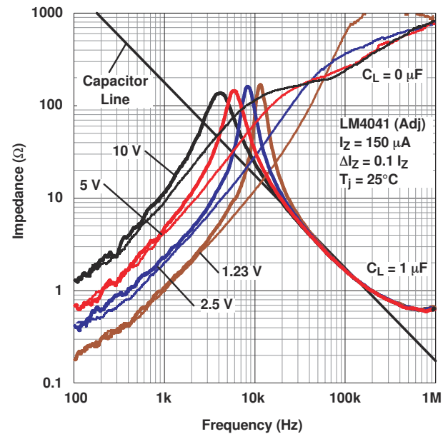
Figure 5-8. Output Impedance vs Frequency
