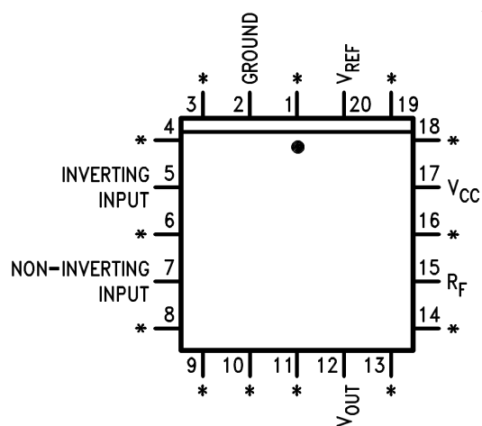
Figure 1. Top View PLCC Package See Package Number FN0020A
