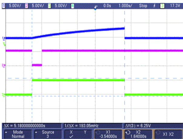
Figure 8-2. \overline{\text{TRIGGER}} , Capacitor Voltage, and OUTPUT Waveforms in Monostable Mode
