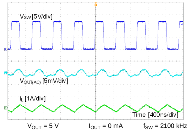
Figure 26. FPWM Mode
