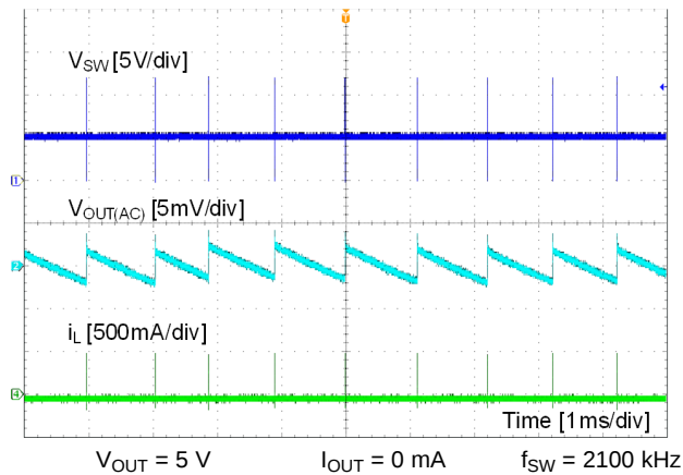
Figure 25. PFM Mode
