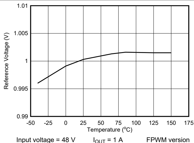
Figure 6-4. Reference Voltage vs Temperature
