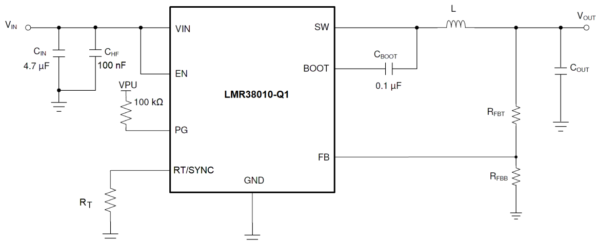
Figure 8-1. Example Application Circuit
