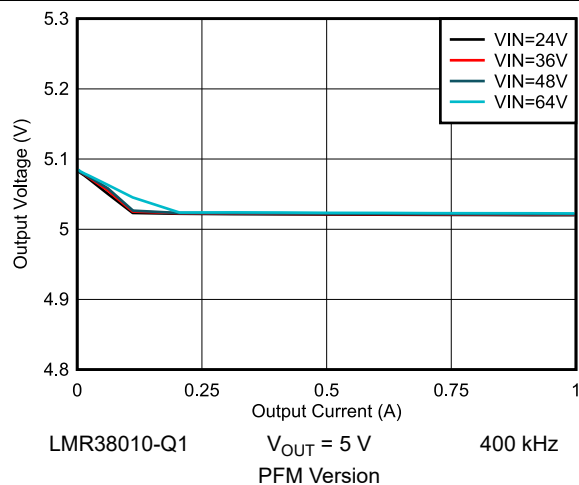
Figure 8-13. 5-V Load Regulation
