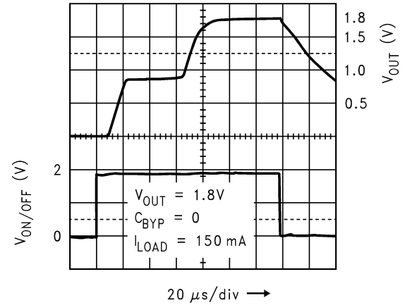
Figure 32. Turnon Time
