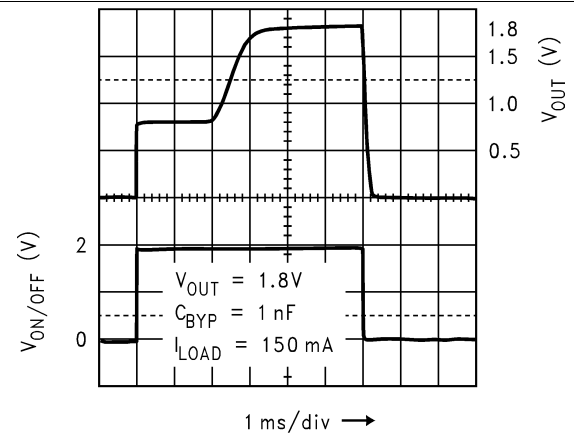
Figure 32. Turnon Time
