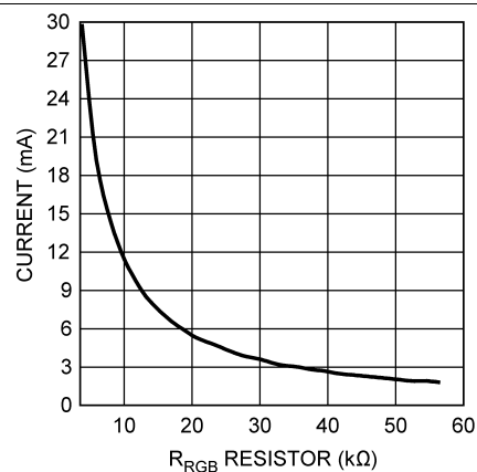
Figure 9. Output Current vs R_{RGB} (Current Sink Mode)
