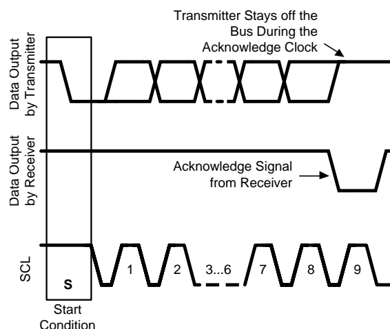
Figure 21. Acknowledge Signal
