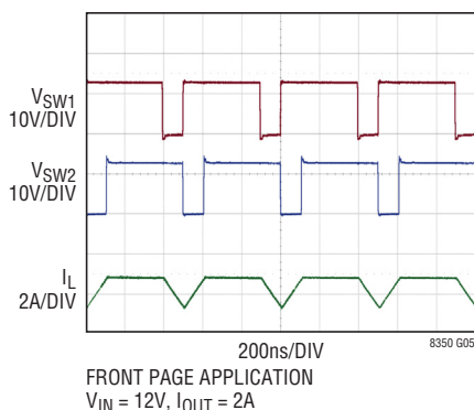
Switching Waveforms (Buck-Boost Region)
