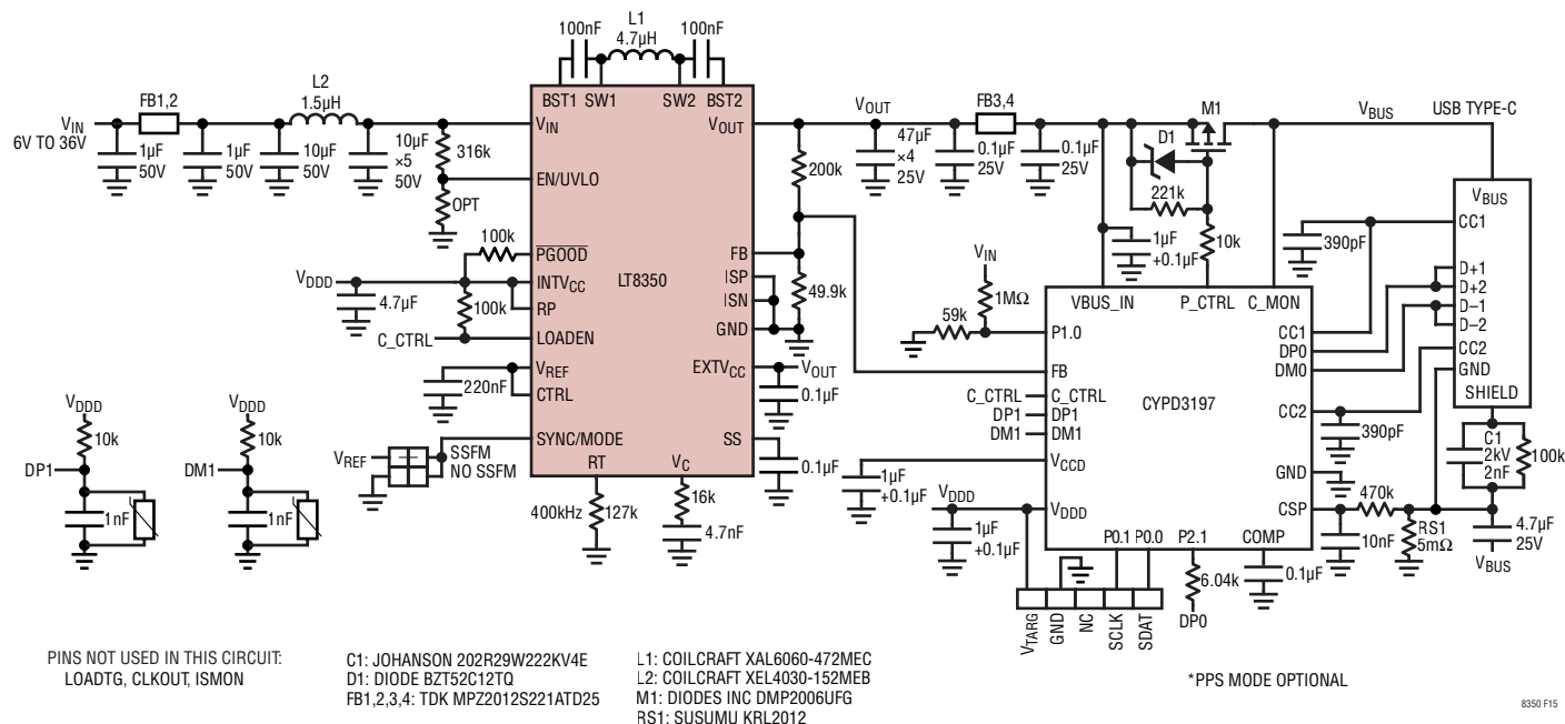
Figure 15. USB-PD Source – 27W 5V, 9V/3A Fixed PDO Mode
