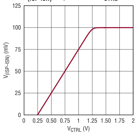
V_{\text{(ISP-ISN)}} Regulation vs V_{\text{CTRL}}
