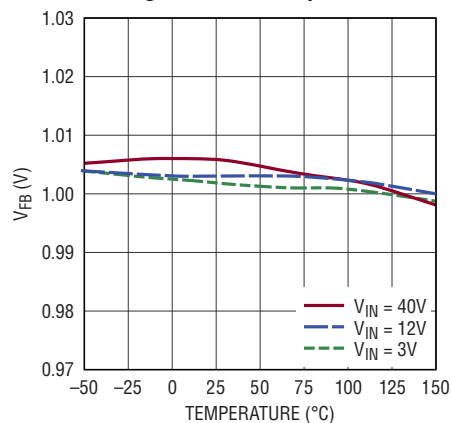
FB Regulation vs Temperature
