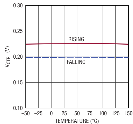
CTRL Off Threshold
