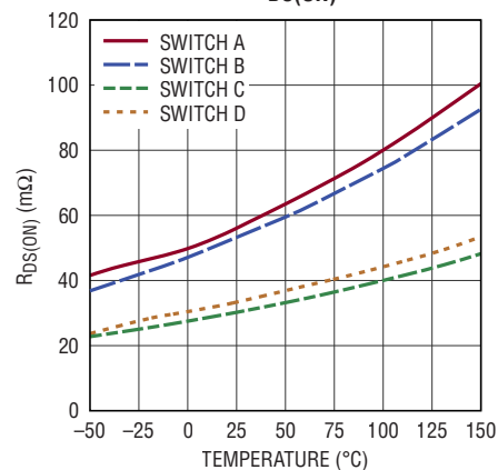
Power Switch R_{\text{DS(ON)}}
