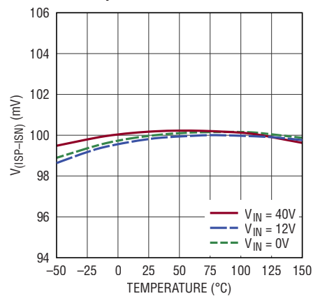
V_{\text{(ISP-ISN)}} Regulation vs Temperature
