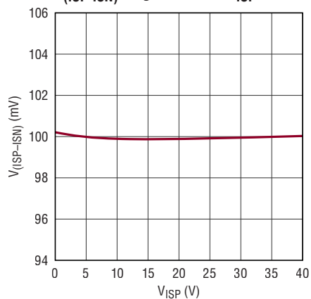
V_{\text{(ISP-ISN)}} Regulation vs V_{\text{ISP}}
