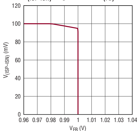
V_{\text{(ISP-ISN)}} Regulation vs V_{\text{FB}}
