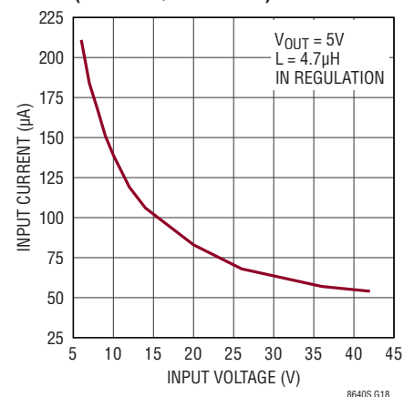
No-Load Supply Current (LT8643S/LT8643SA)
