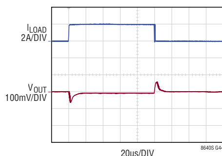
Transient Response; External Compensation (LT8643S/LT8643SA)
