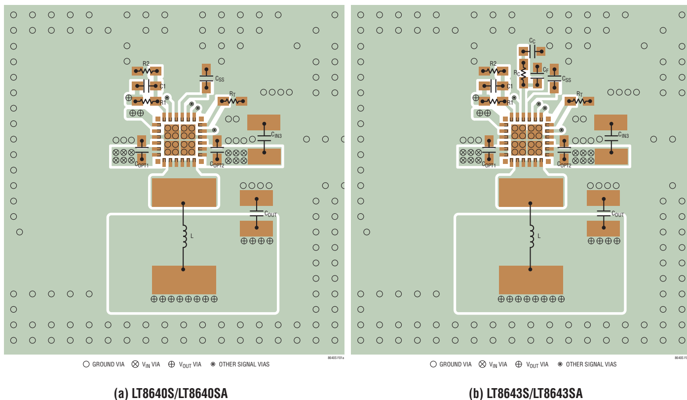
Figure 1. Recommended PCB Layouts for the LT8640S/LT8640SA and LT8643S/LT8643SA
