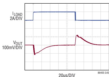
Transient Response; Internal Compensation (LT8640S/LT8640SA)
