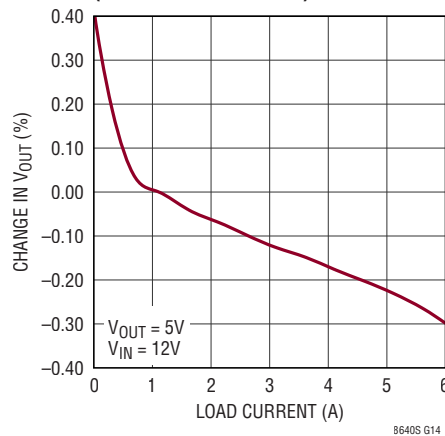
Load Regulation (LT8643S/LT8643SA)
