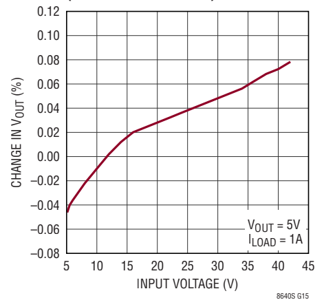
Line Regulation (LT8640S/LT8640SA)
