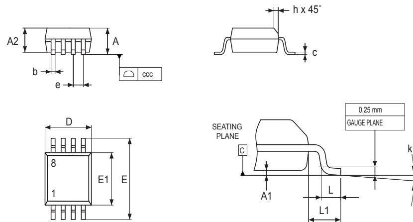
Figure 24. SO8N - Outline
