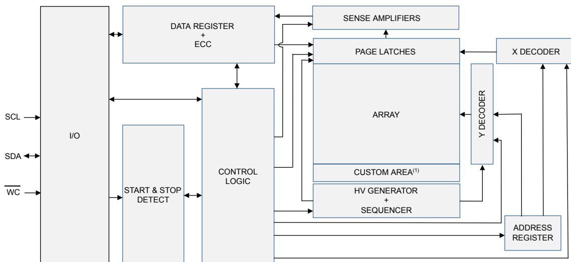
Figure 4. Block diagram
