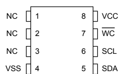
Figure 3. 8-pin package connections, top view
