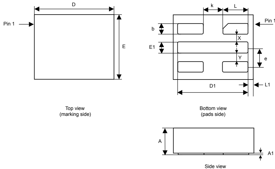
Figure 30. UFDFPN5 - Outline
