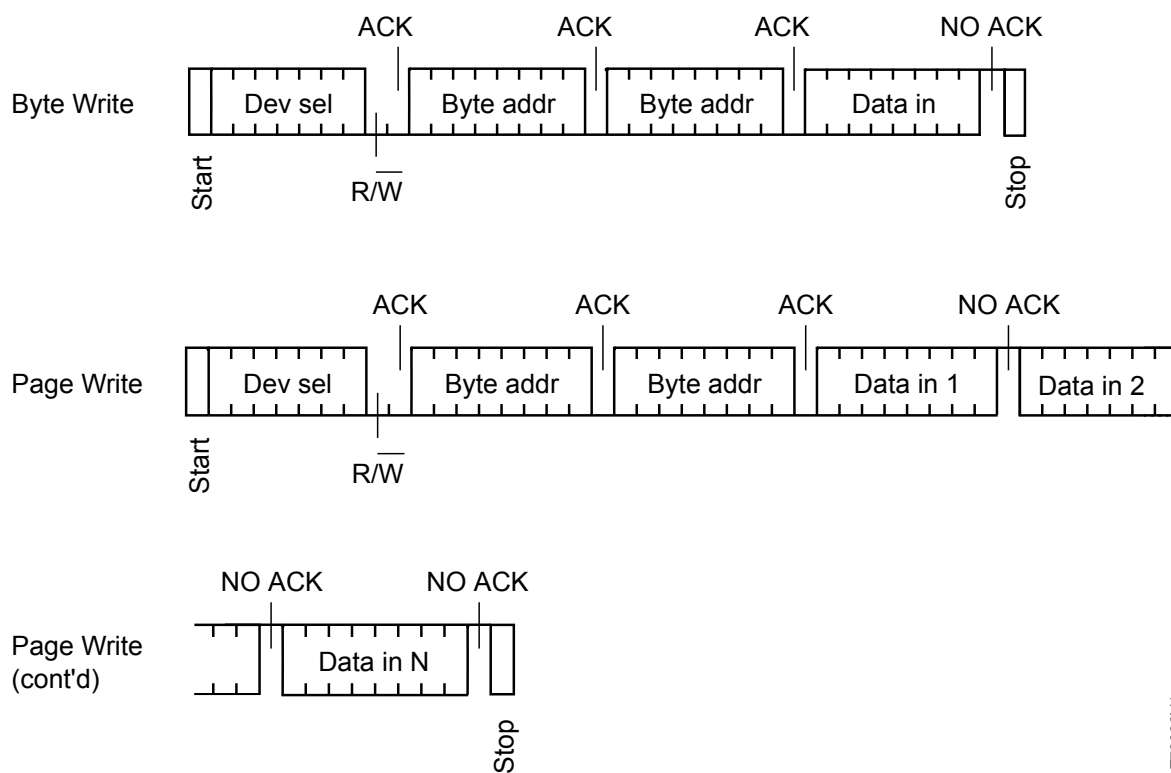
Figure 11. Write identification page (page locked or hard protected)
