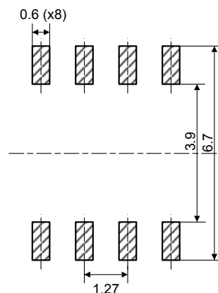
Figure 25. SO8N - Footprint example
