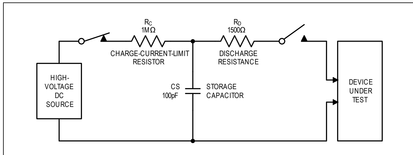
Figure 44. Human Body ESD Test Model
