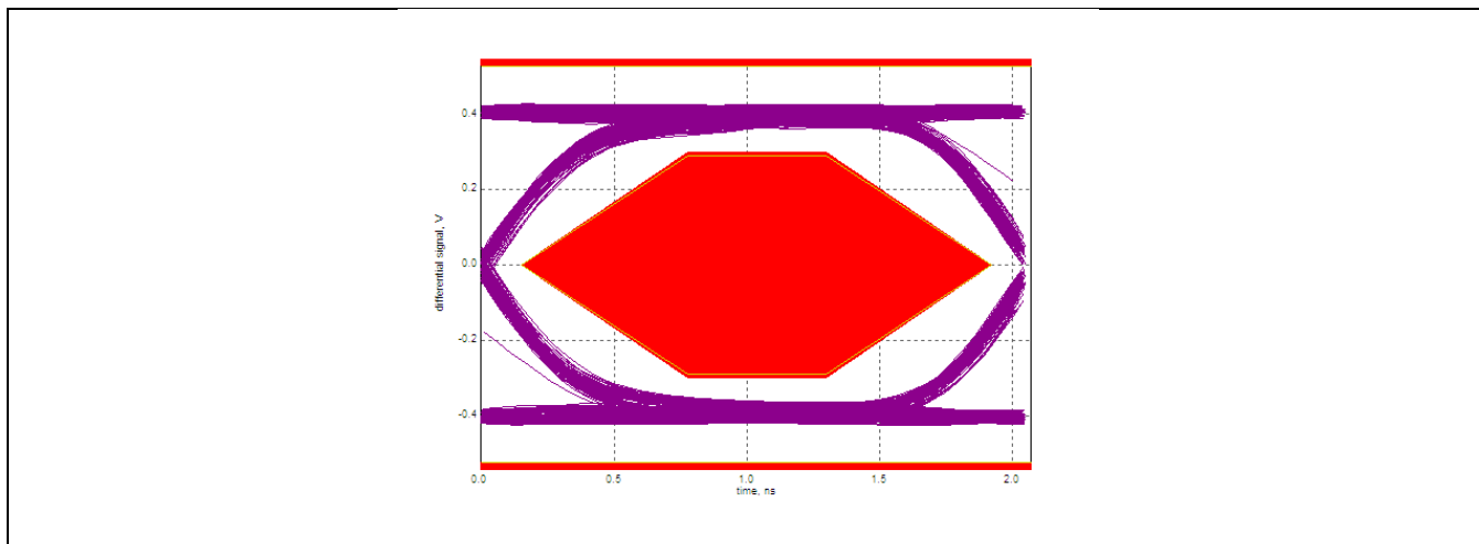
Figure 43. Untuned Near-Eye Diagram (with MAX25432)
