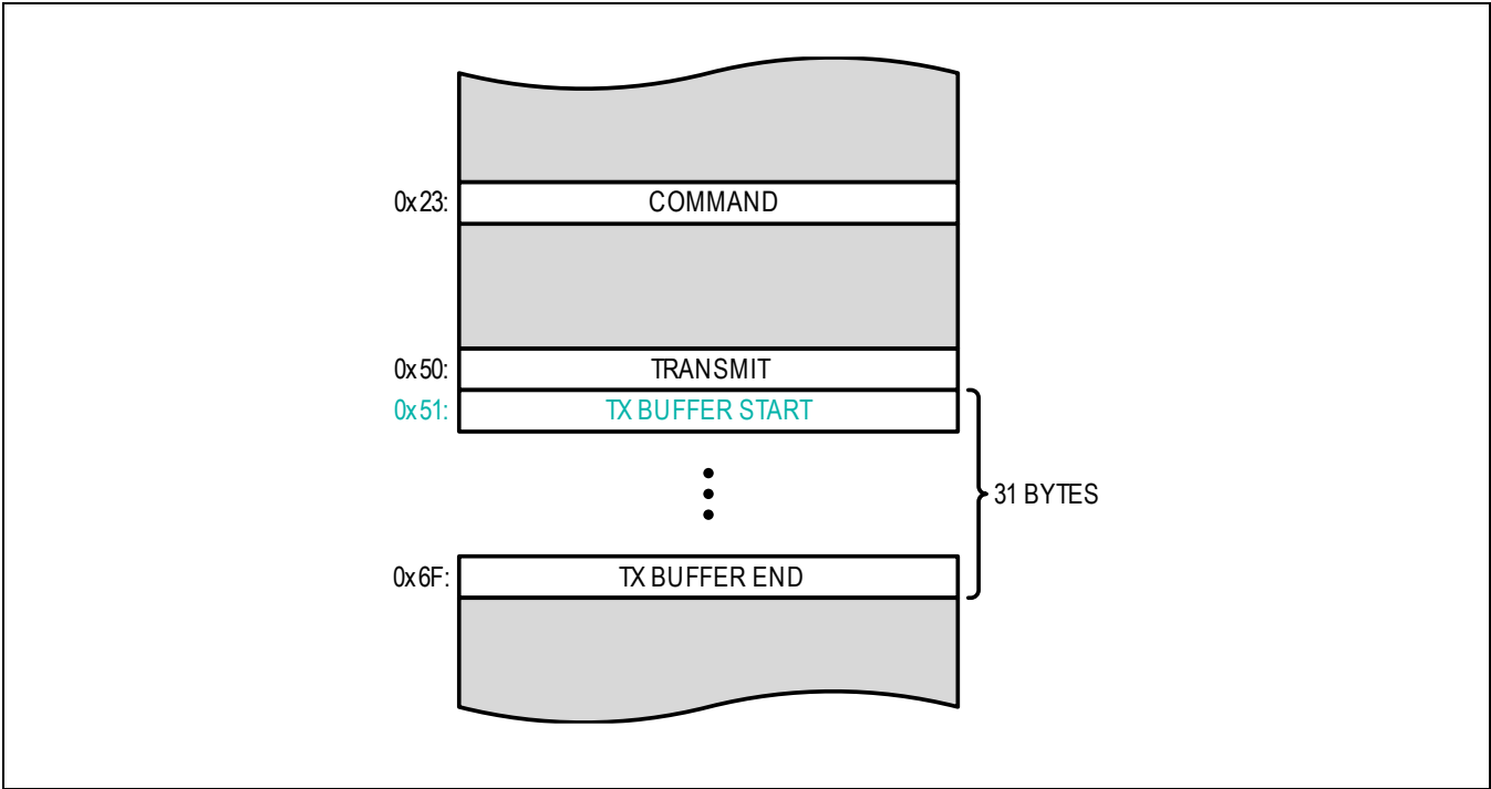
Figure 33. Transmit Buffer
