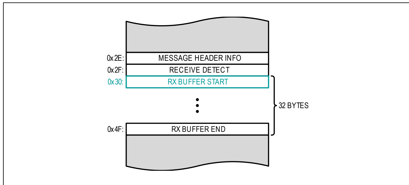
Figure 31. Receive Buffer
