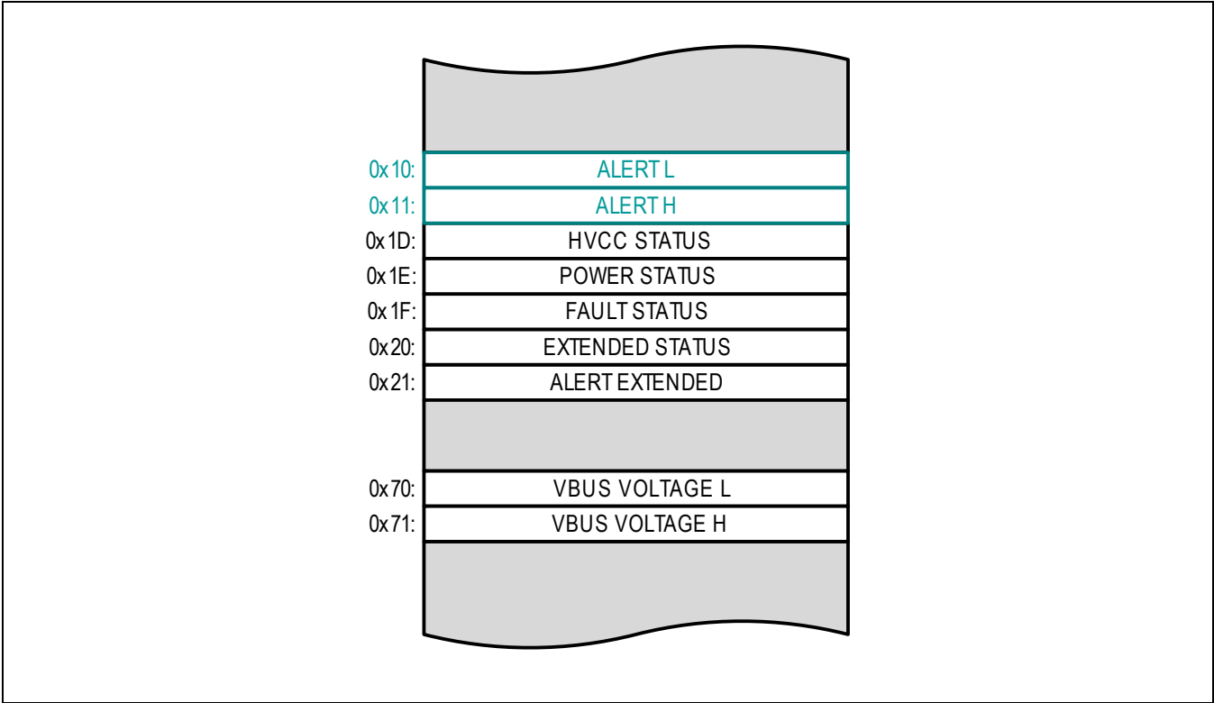
Figure 30. Status Registers
