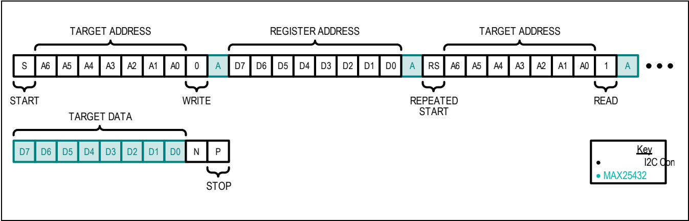
Figure 26. Read Byte
