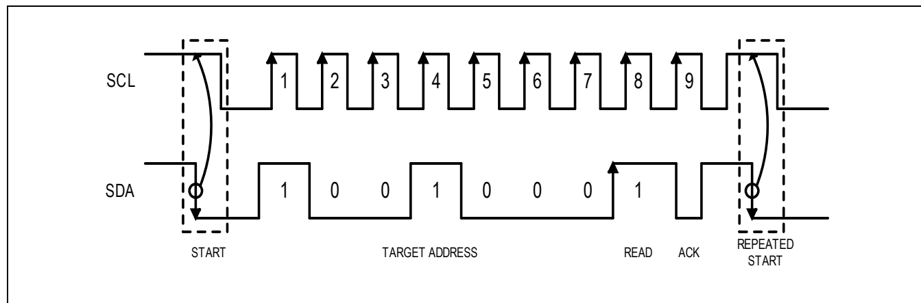
Figure 22. REPEATED START Condition
