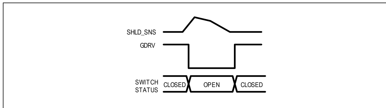
Figure 17. Shield/GND Short-to-Battery Timing Diagram
