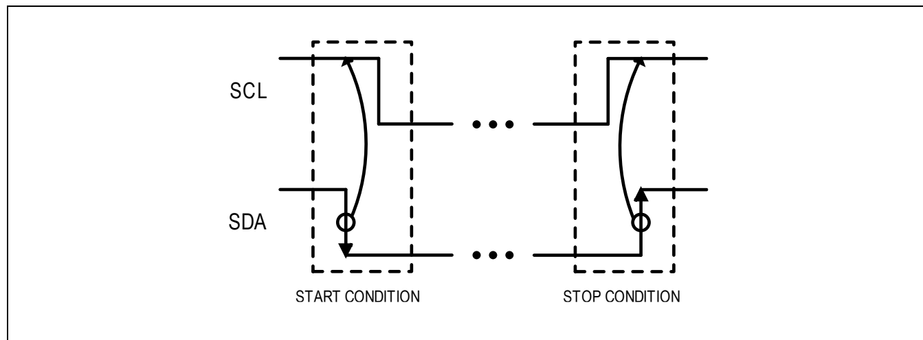
Figure 21. START and STOP Conditions
