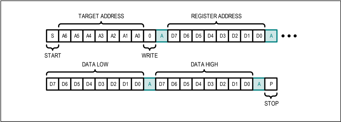
Figure 24. Write Word
