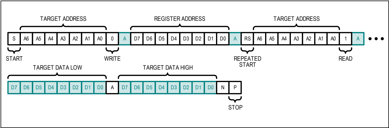
Figure 27. Read Word
