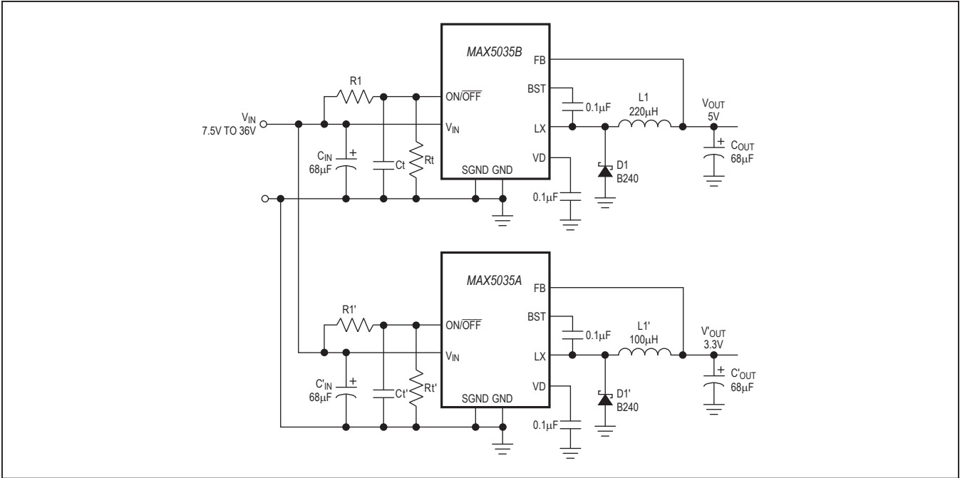
Figure 4. Dual-Sequenced DC-DC Converters (Startup Delay Determined by R1/R1', Ct/Ct' and Rt/Rt')
