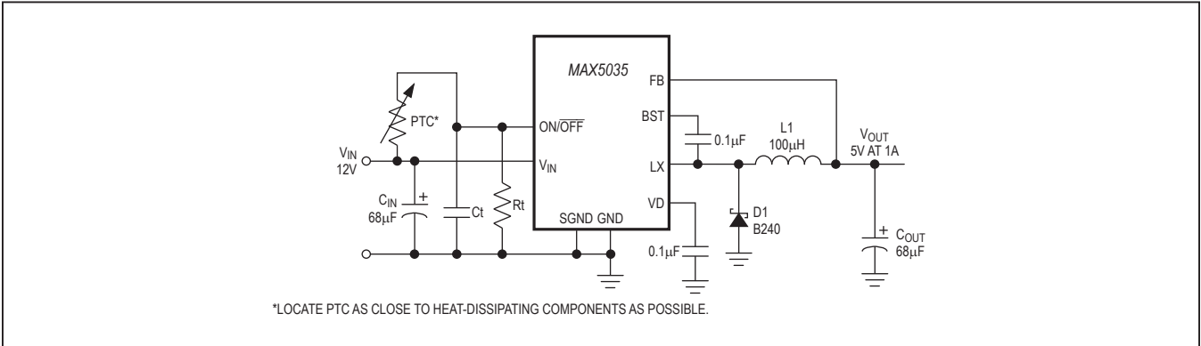
Figure 3. Load Temperature Monitoring with ON/OFF (Requires Accurate VIN)
