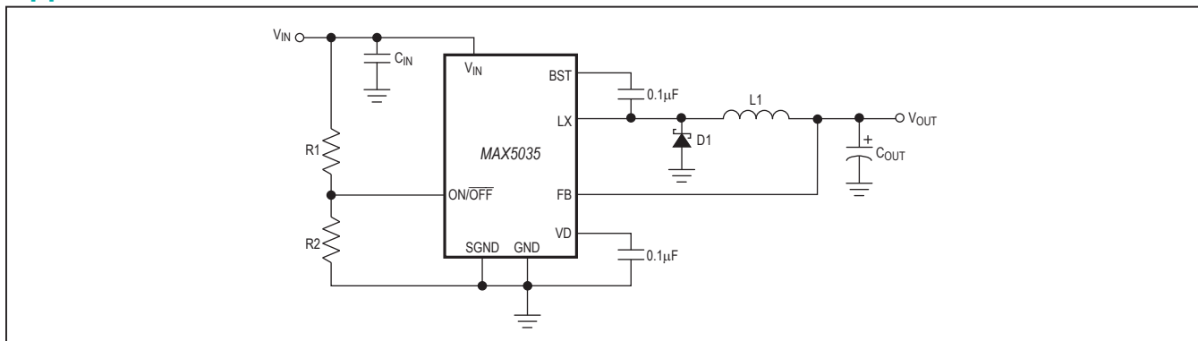
Figure 2. Fixed Output Voltages
