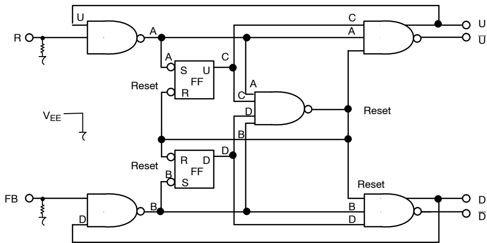
Figure 3. Logic Diagram
