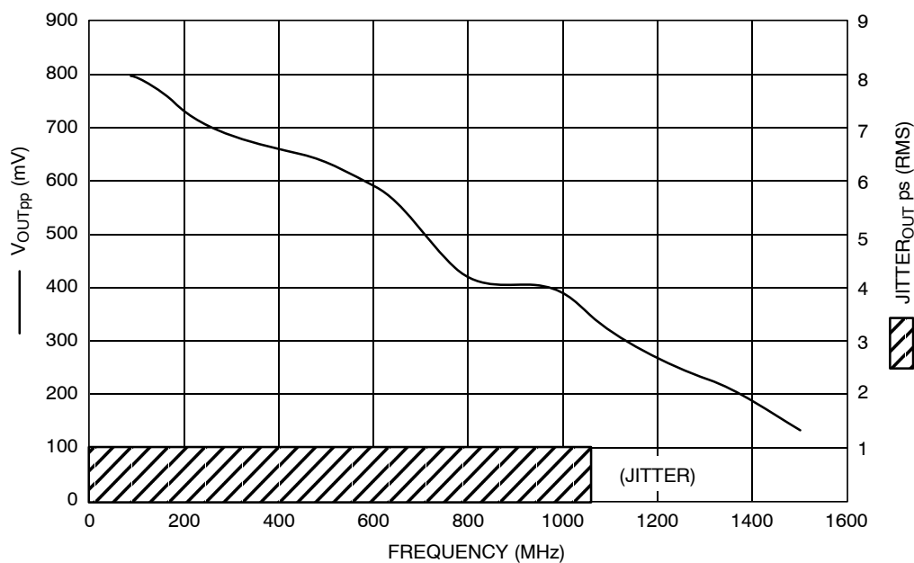
Figure 2. F_{\max} /Jitter
