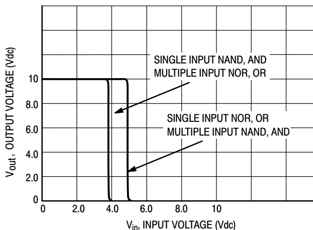
Figure 9. V_{DD} = 10 Vdc
