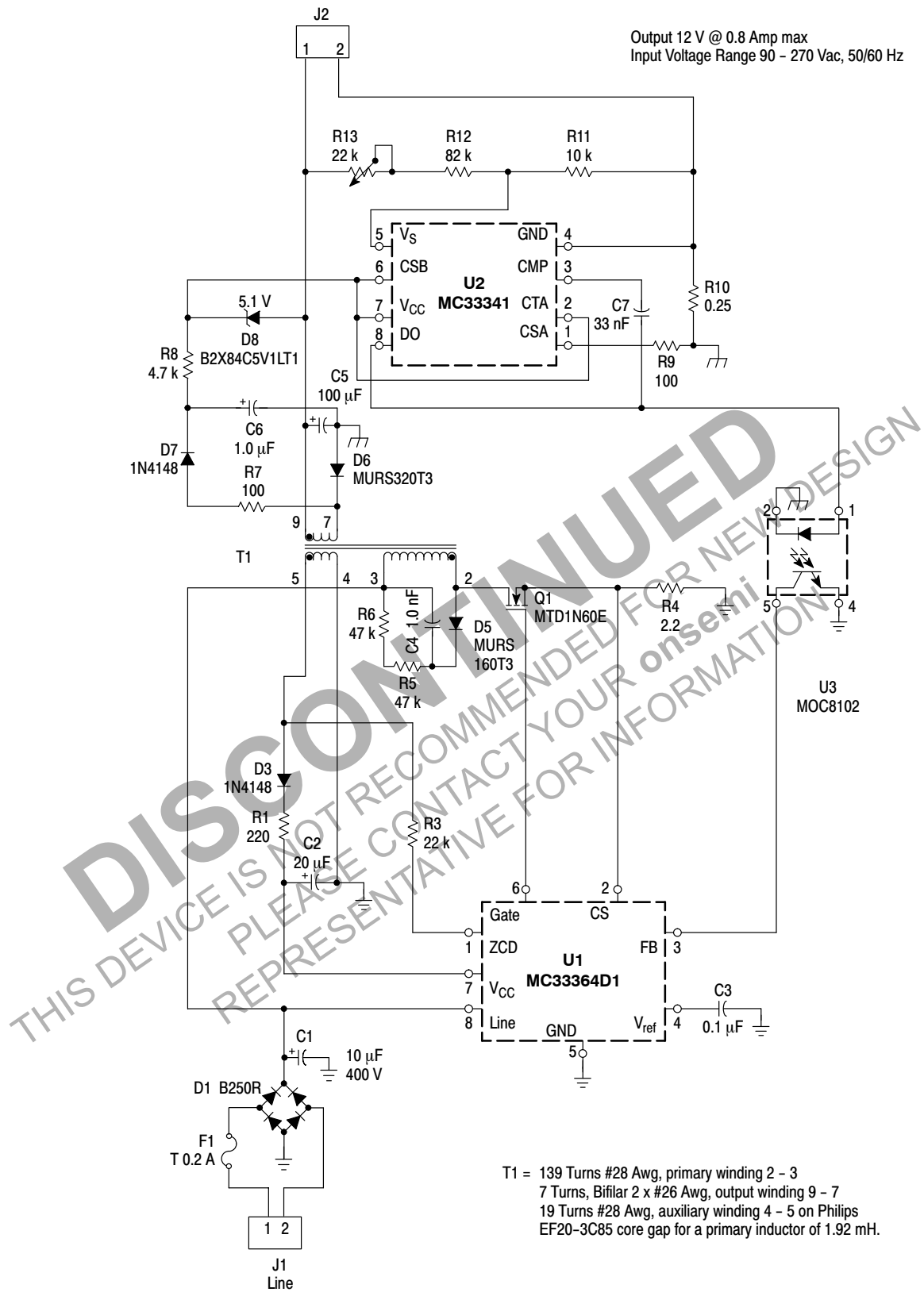
Figure 16. Universal Input Battery Charger
