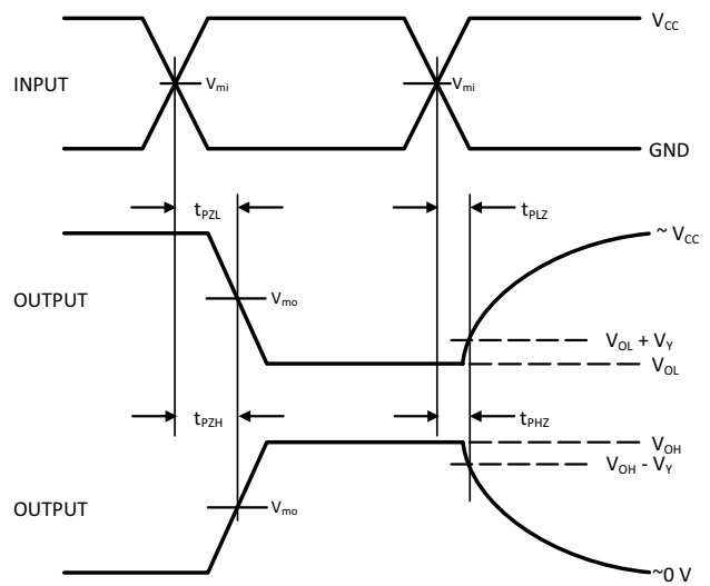
Figure 4. Switching Waveforms
