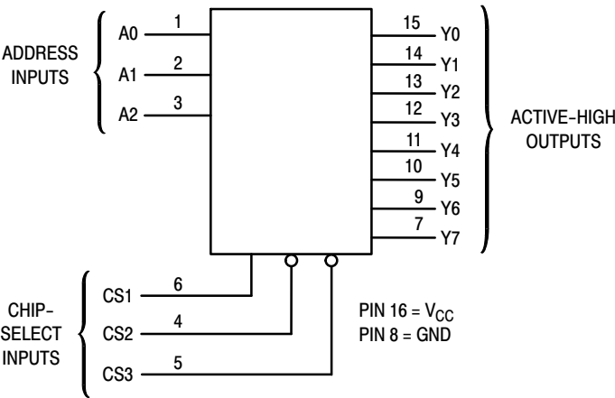
Figure 2. Logic Diagram
