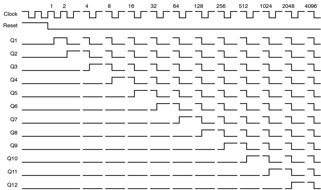
Figure 7. Timing Diagram
