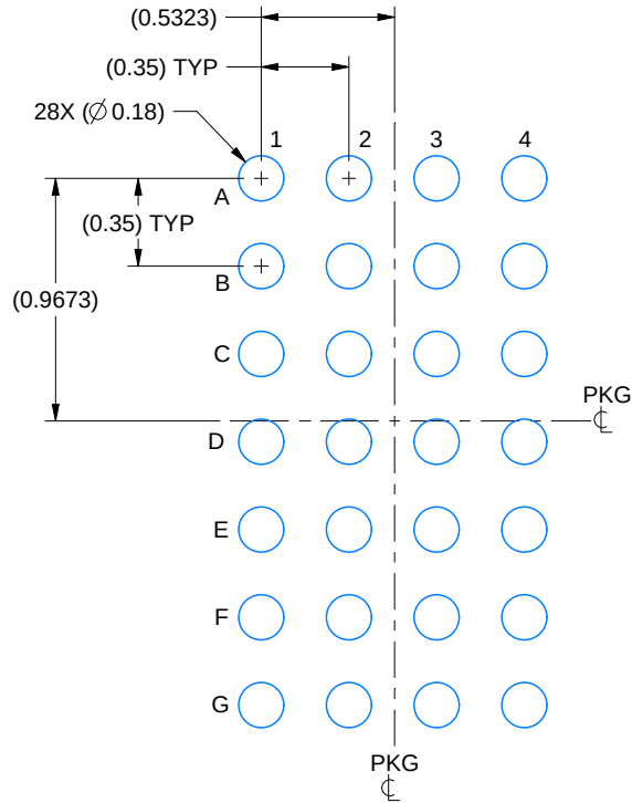
LAND PATTERN EXAMPLE EXPOSED METAL SHOWN SCALE: 30X
