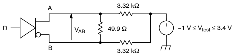
Figure 5. Differential Output Voltage Test Circuit
