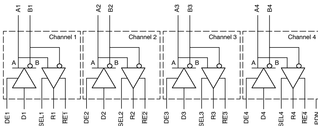
Figure 2. Block Diagram
