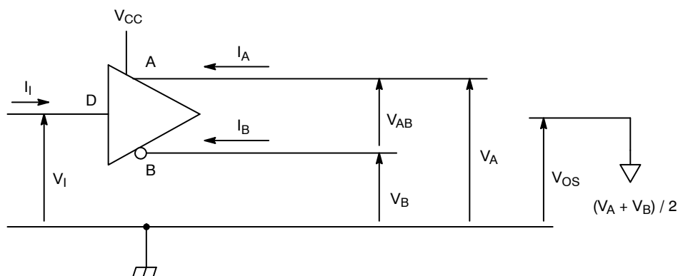
Figure 4. Driver Voltage and Current Definitions
