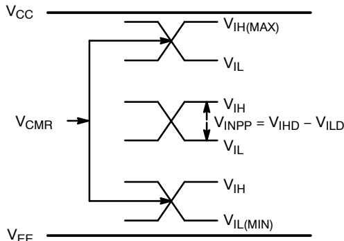
Figure 19. V_{CMR} Diagram
