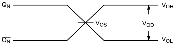
Figure 15. LVDS Output
