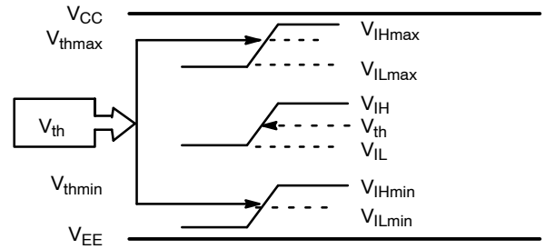
Figure 5. V_{th} Diagram
