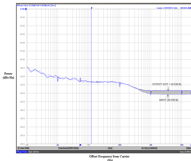
Figure 8. Typical Phase Noise Plot at f_{\text{carrier}} = 2 \text{ GHz}
