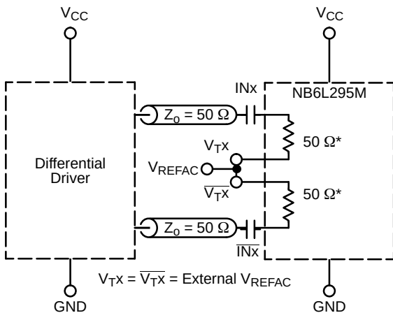
Figure 20. Capacitor-Coupled Differential Interface ( V_{TX}/\overline{V_{TX}} Connected to V_{REFAC} ; V_{REFAC} Bypassed to Ground with 0.1\ \mu\text{F} Capacitor)
