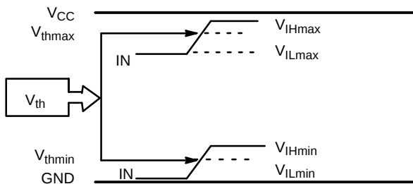
Figure 21. V_{th} Diagram
