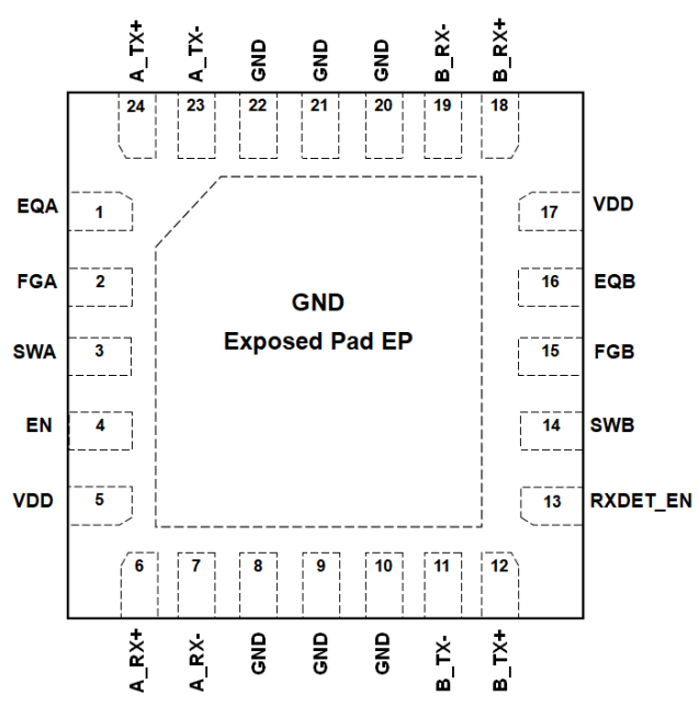
Figure 2. UQFN24 Package Pinout (Top View)
